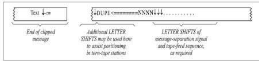
Figure 4-3. Example of application of 23.2.4.4.11.3 procedure
